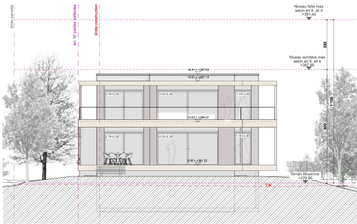
FACADE SUD
